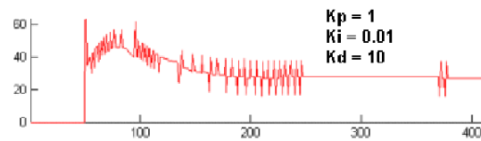
Asservissement PID
